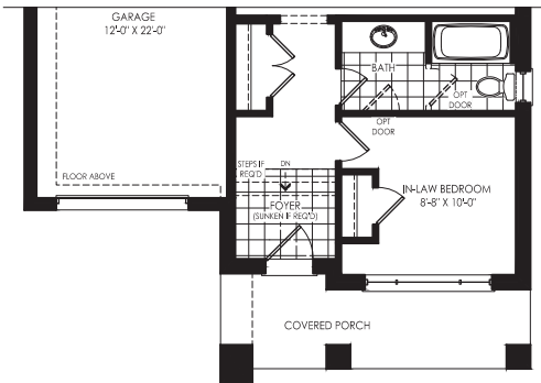
ELEVATION B OPTIONAL GROUND LEVEL
