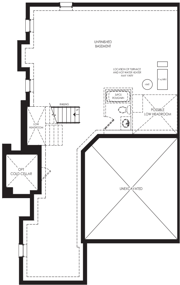
ELEVATION A BASEMENT
