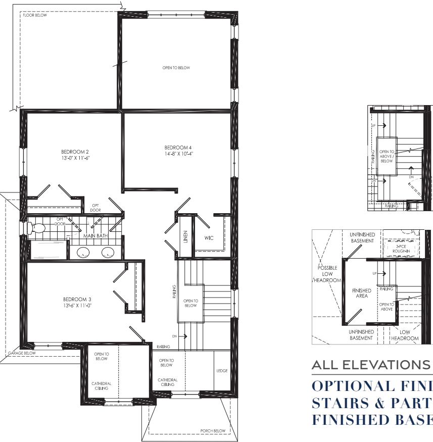
ELEVATION A OPTIONAL SECOND LEVEL 4 BEDROOM PLAN
