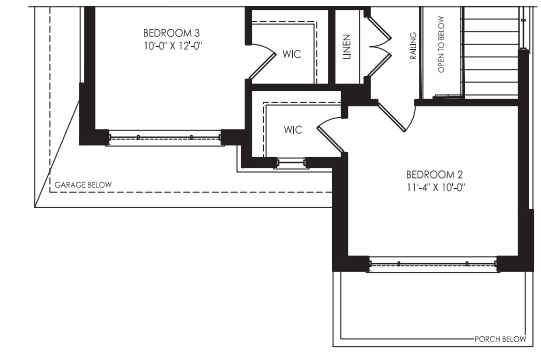
ELEVATION B SECOND LEVEL
