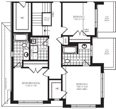
ELEVATION B OPTIONAL SECOND LEVEL
