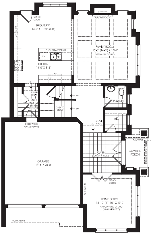
ELEVATION A GROUND LEVEL
