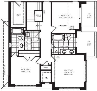
ELEVATION B SECOND LEVEL
